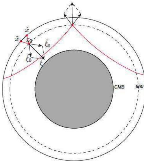
FIG. 1. Scattered rays (broken geodesics) for imaging discontinuities (here the “660” corresponding with a phase transition at 660 km depth) in Earth’s mantle. (CMB stands for core-mantle boundary.)
