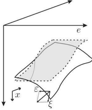
FIG. 2. Wavefront set of an extended image, r = r(x, e) . The gray surface (singular support) corresponds with \varepsilon = 0 and maps into the range of the scattering operator before extension. The transparent surface exemplifies the extension to \varepsilon values away from zero.
